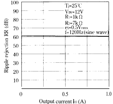
Fig.14 Ripple Rejection vs. Output Current (PQ20VZ11)
